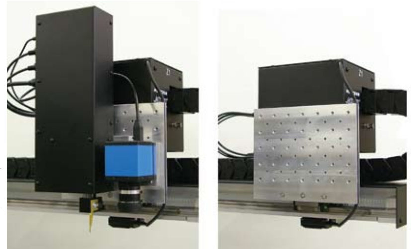
Left image - probe head assembly with Z axis probe head and camera mounted Right Image - special adapter plate that allows for complete head customization
